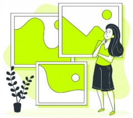
Inference
